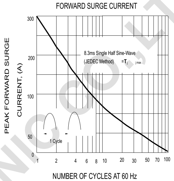
FIG.2-MAXIMUM NON-REPETITIVE PEAK
