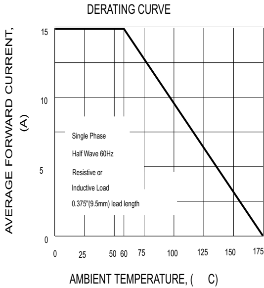
FIG.1-TYPICAL FORWARD CURRENT
